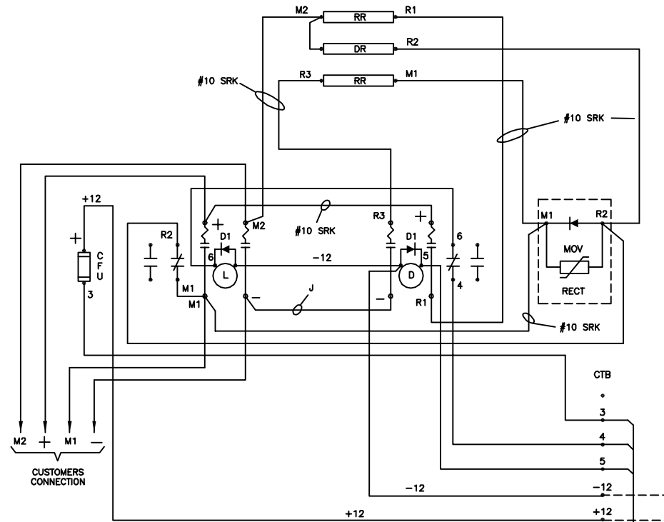
FRONT VIEW CONNECTION DIAGRAM
